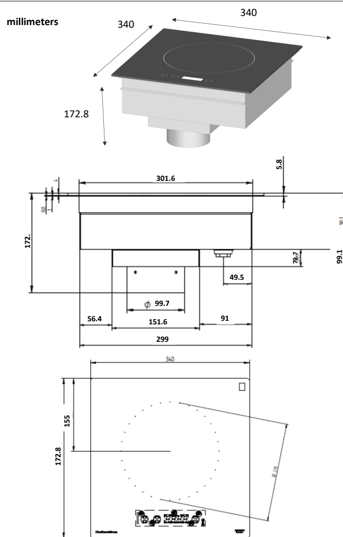
Cut out dimensions 346x346mm
