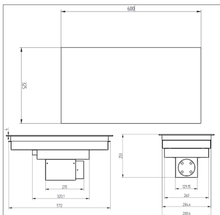
Dimensions of the integration of the cooking block: 606x331mm
